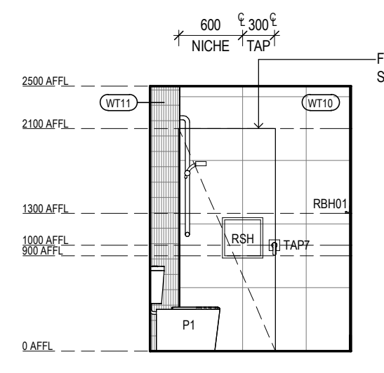
ILA BT-04 ELEVATION 4 Scale 1: 50
