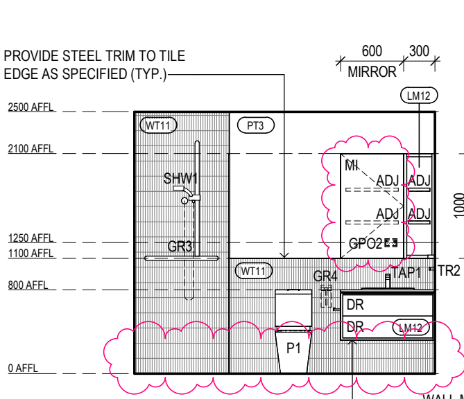
ILA BT-03 ELEVATION 1 Scale 1: 50
