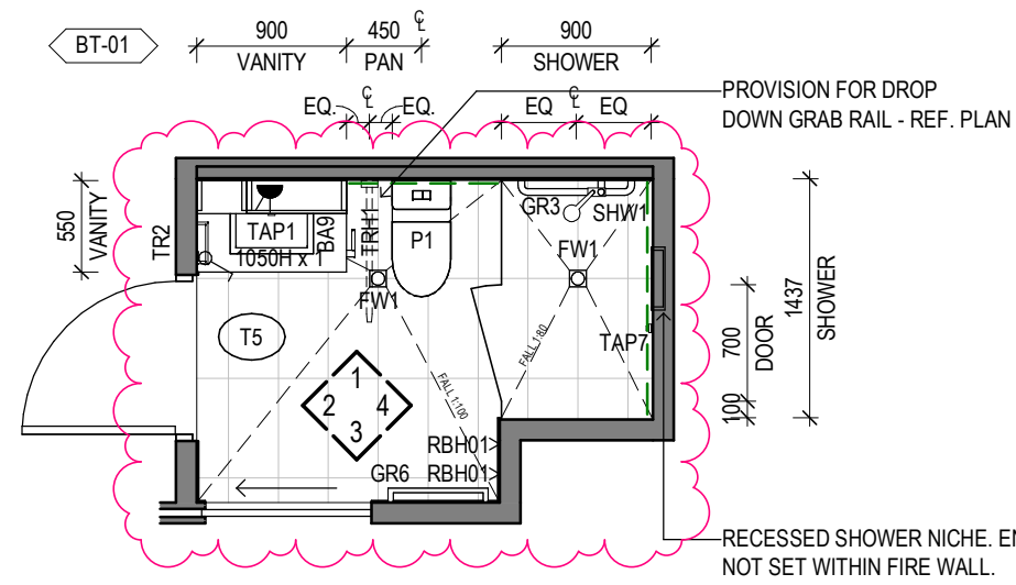
1 ILA BT-01 Scale 1: 50
