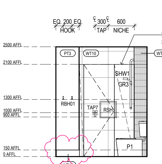
ILA BT-03 ELEVATION 2 Scale 1: 50
