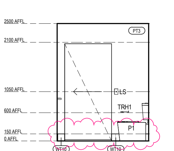
ILA BT-02 ELEVATION 2 Scale 1: 50
