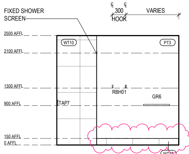
ILA BT-04 ELEVATION 3 Scale 1: 50
