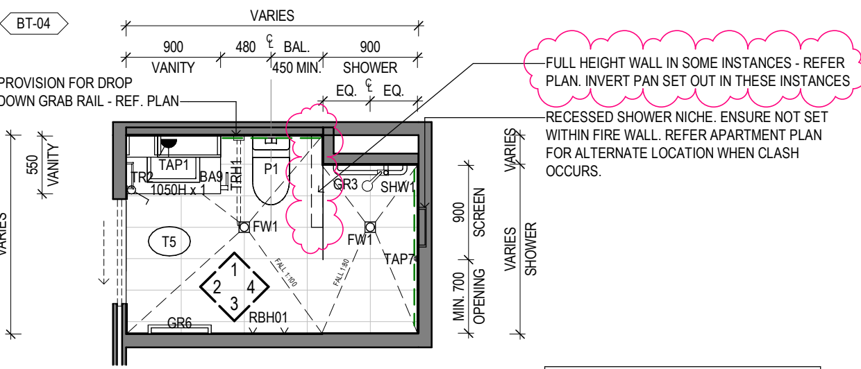
4 ILA BT-04 Scale 1: 50
