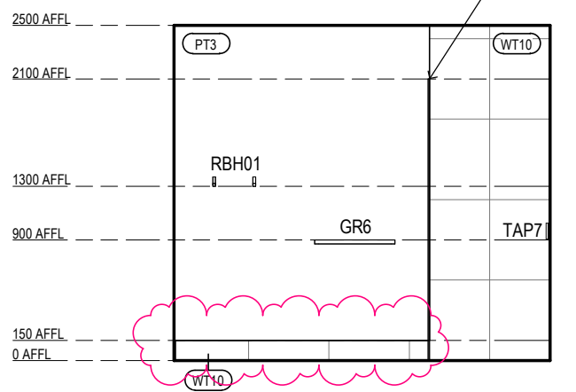
ILA BT-05 ELEVATION 3 Scale 1: 50
