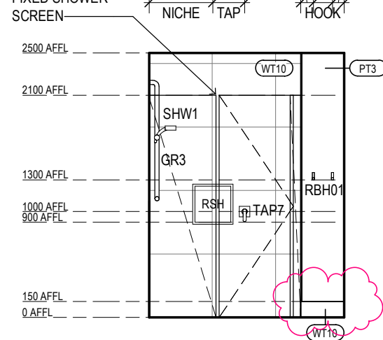
ILA BT-02 ELEVATION 4 Scale 1: 50
