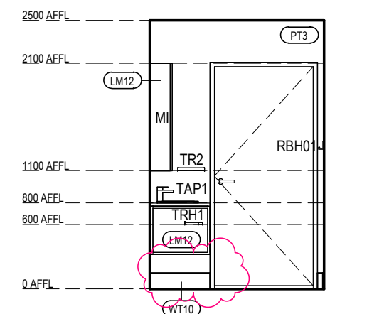
ILA BT-05 ELEVATION 4 Scale 1: 50
