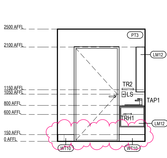
ILA BT-01 ELEVATION 2 Scale 1: 50
