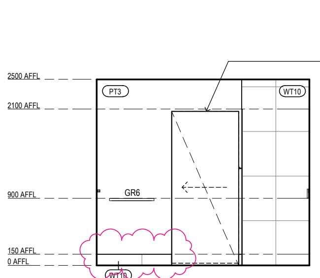
ILA BT-03 ELEVATION 3 Scale 1: 50
