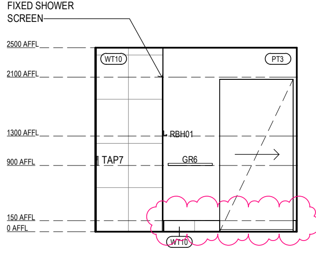
ILA BT-01 ELEVATION 3 Scale 1: 50
