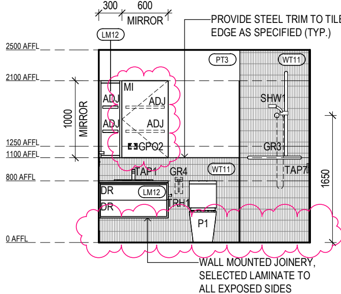
ILA BT-01 ELEVATION 1 Scale 1: 50
