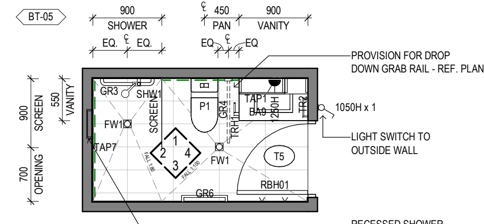
5 ILA BT-05 Scale 1: 50
