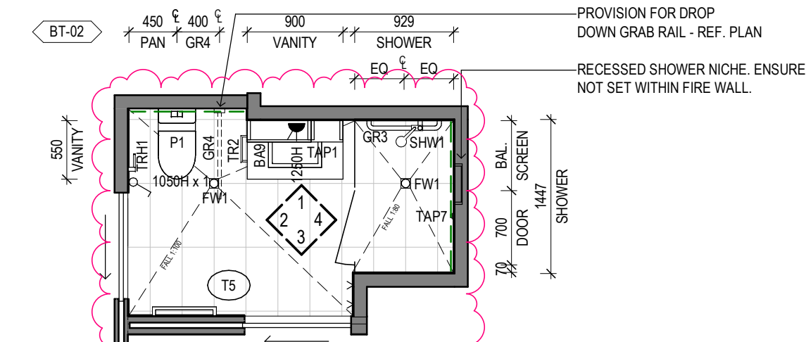
2 ILA BT-02 Scale 1: 50
