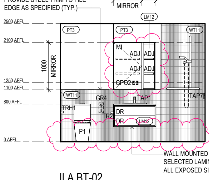
ILA BT-02 ELEVATION 1 Scale 1: 50
