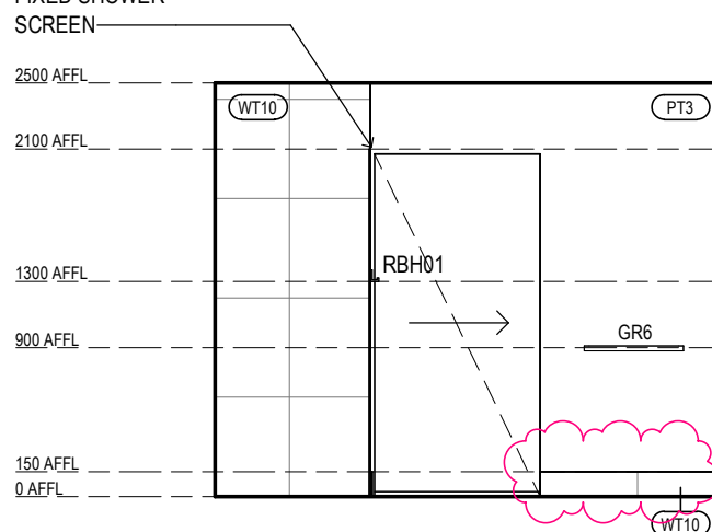
ILA BT-02 ELEVATION 3 Scale 1: 50
