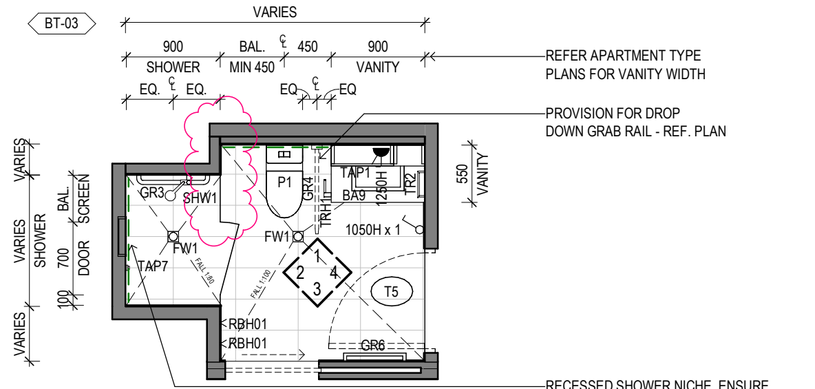
3 ILA BT-03 Scale 1: 50
