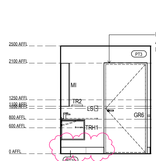
ILA BT-03 ELEVATION 4 Scale 1: 50
