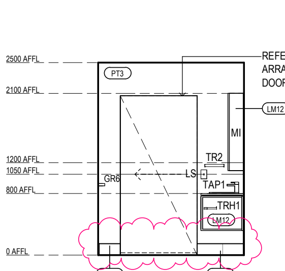
ILA BT-04 ELEVATION 2 Scale 1: 50
