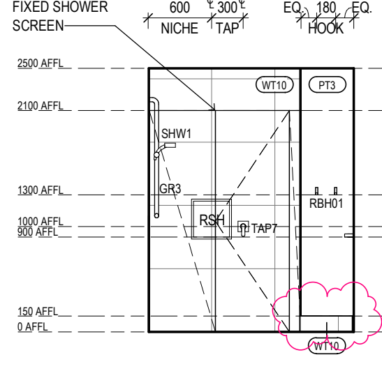
ILA BT-01 ELEVATION 4 Scale 1: 50
