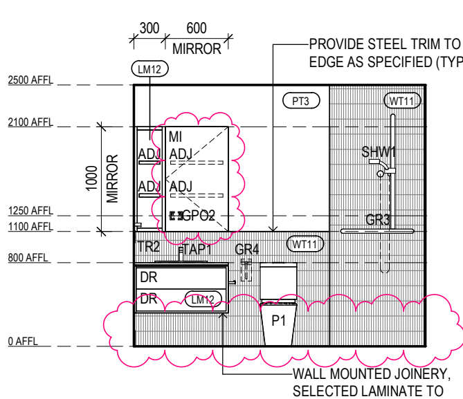
ILA BT-04 ELEVATION 1 Scale 1: 50
